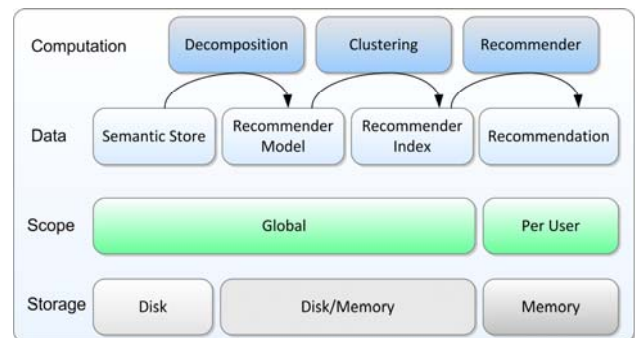
Figure 4 Detailed view of the SmartSenior recommender. Recommendations are computed using a three-stage algo-
