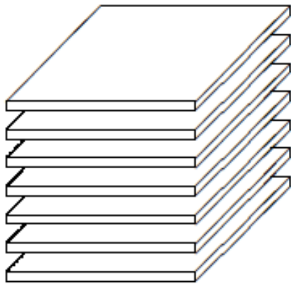
(a) Horizontal slices: \mathbf{X}_{i::}
